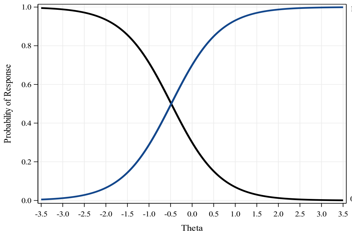
Figure 6.1. Two-Parameter Item Response Functions for a Mathematics Item from ISASP Grade 5
