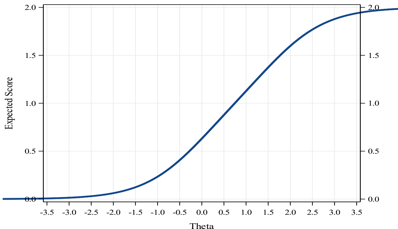
Figure 6.3. Two-Parameter Graded Response Model Expected Item Score Function for a Constructed-Response Mathematics Item from ISASP Grade 8
